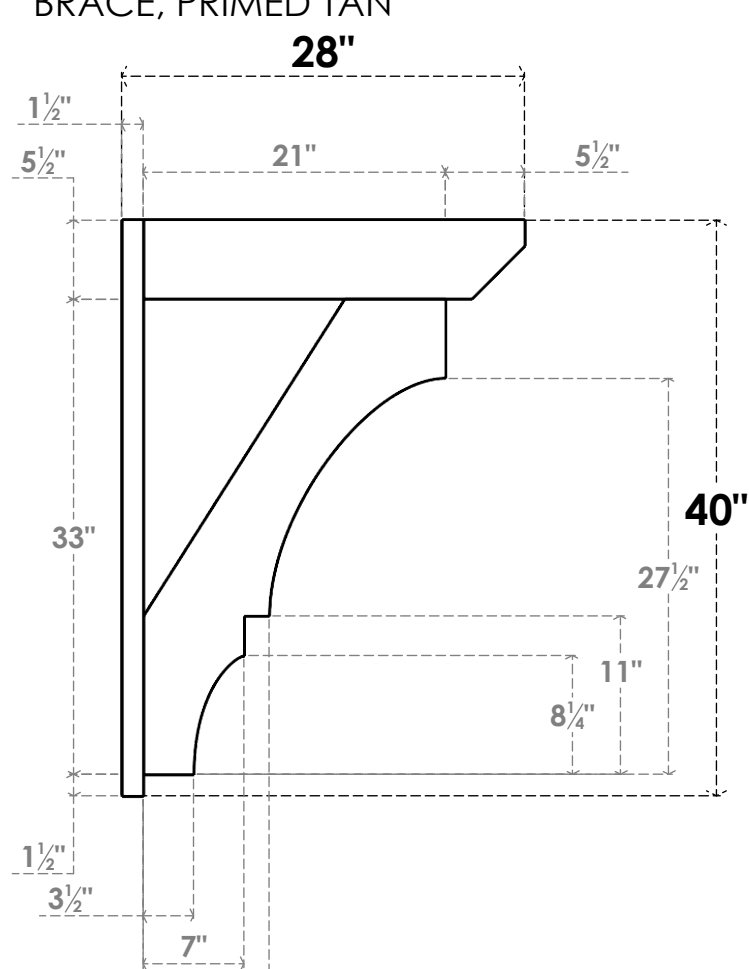
SIDE PROFILE
